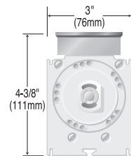
C. MECHO/5 POCKET DRIVE-END BRACKET
