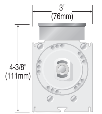
C. MECHO/5 POCKET DRIVE-END BRACKET
