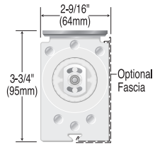
A. MECHO/5 SLIMLINE DRIVE-END BRACKET
