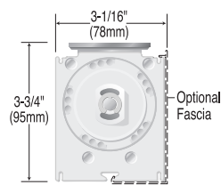
B. MECHO/5 STANDARD DRIVE-END BRACKET
