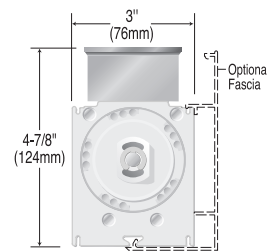
D. MECHO/5 EXTENDED DRIVE-END BRACKET
